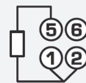
3-wire RTD
